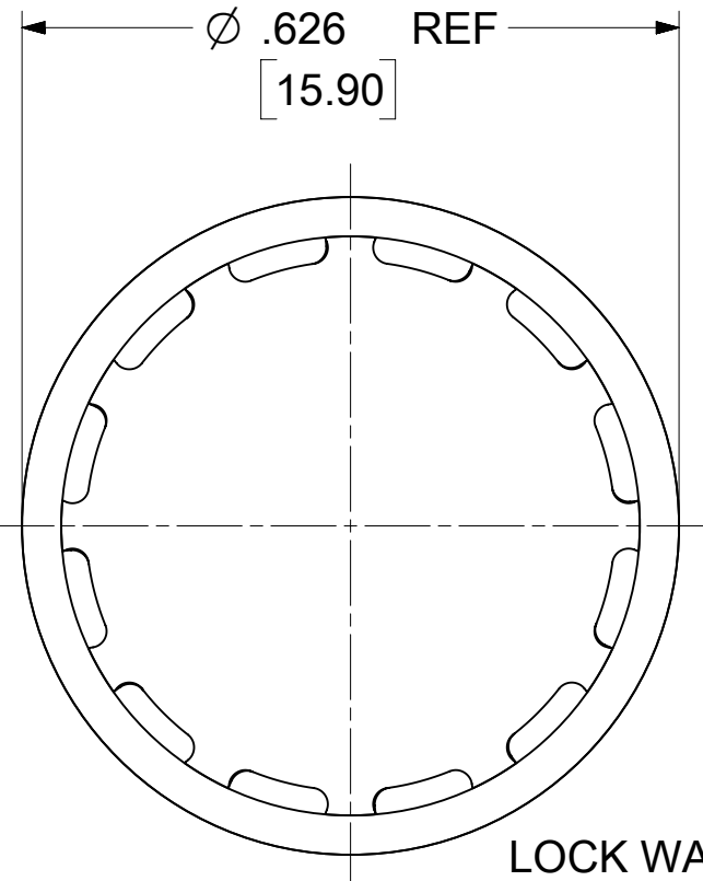
LOCK WASHER
