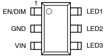
CAT4003B TSOT23-6L, TSOP-6
