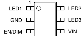
CAT4003B SC70-6L
