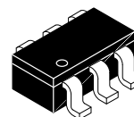
TSOT23-6 TD SUFFIX CASE 419AF
