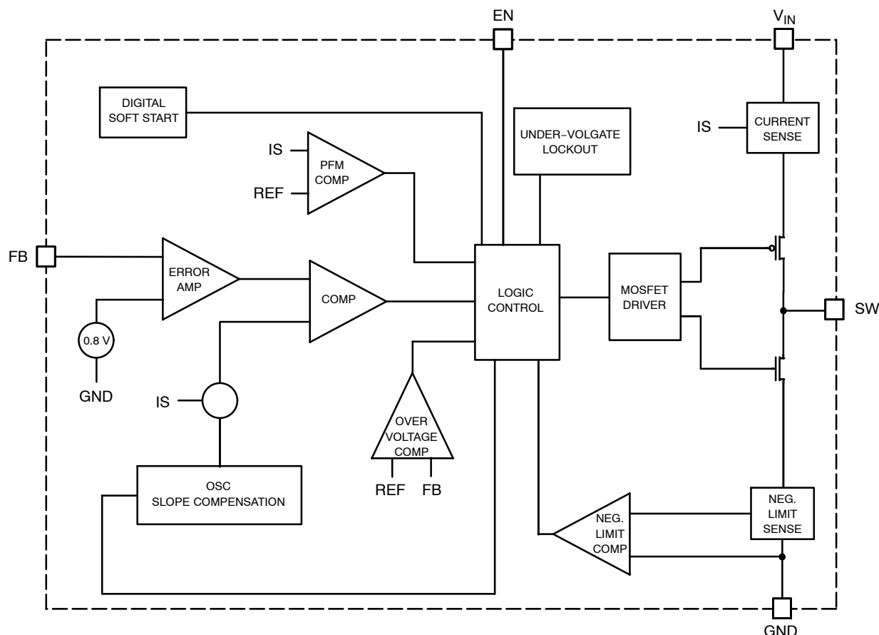
Figure 15. Block Diagram
