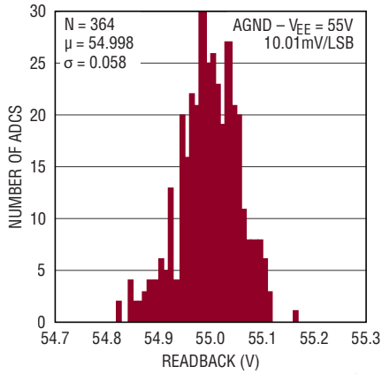
V EE Readback
