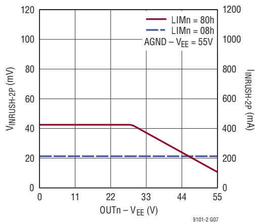
Inrush Current Limit (Note 16)
