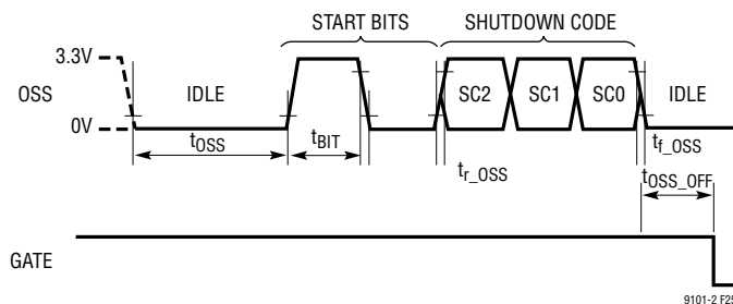
Figure 25. Multi Bit Priority Port Shutdown of Lower-Priority Port
