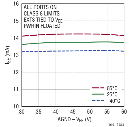
V EE Supply Current vs Voltage and Temperature
