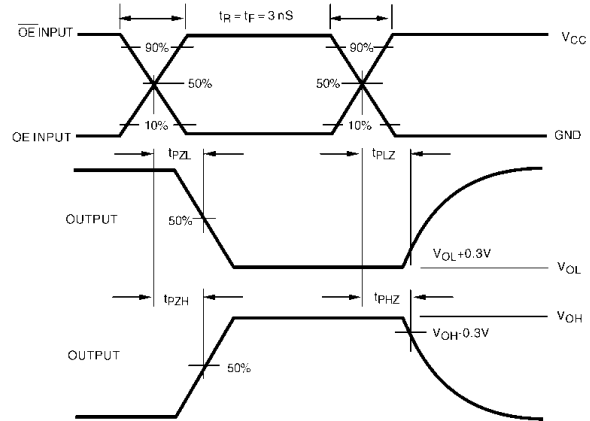
Figure 7. AC Waveforms
