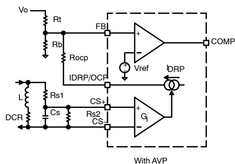
Figure 24. OCP Configuration
