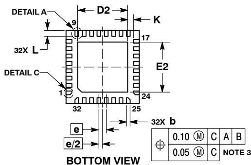
DETAIL C 4 PLACES
