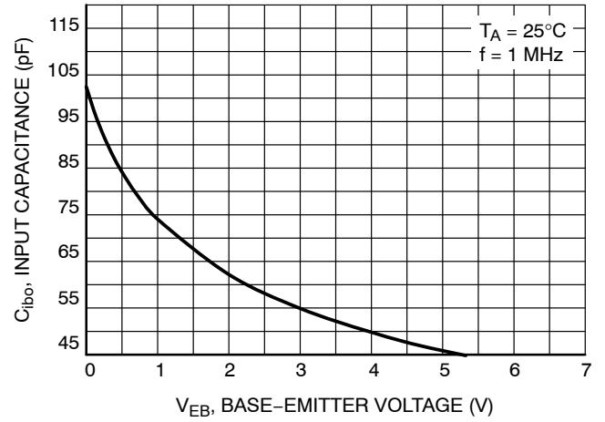
Figure 10. Input Capacitance
