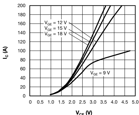
Fig. 2 - Typical Trench IGBT Output Characteristics, T_J = 125 °C
