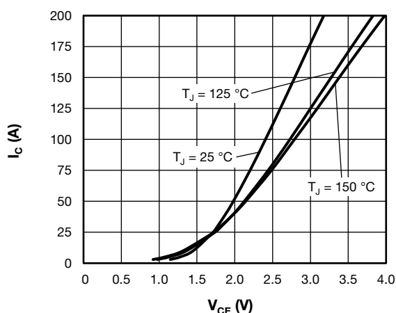
Fig. 1 - Typical Trench IGBT Output Characteristics, V_{GE} = 15 V
