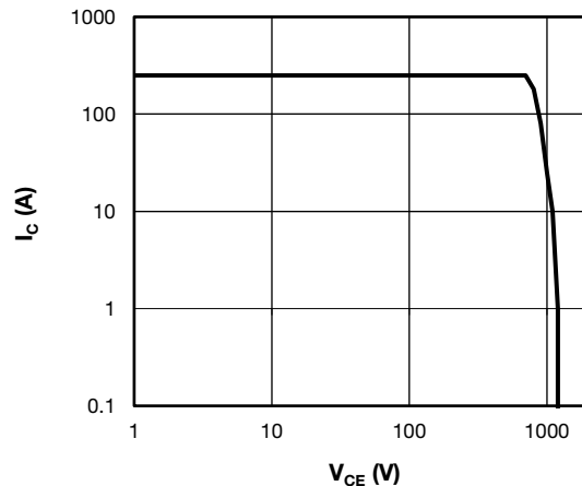
Fig. 16 - Trench IGBT Reverse BIAS SOA T_J = 150 \text{ °C} , I_C = 250 \text{ A} , R_g = 10 \text{ Ω} , V_{GE} = +15 \text{ V/0 V} , V_{CC} = 700 \text{ V} , V_p = 1200 \text{ V}
