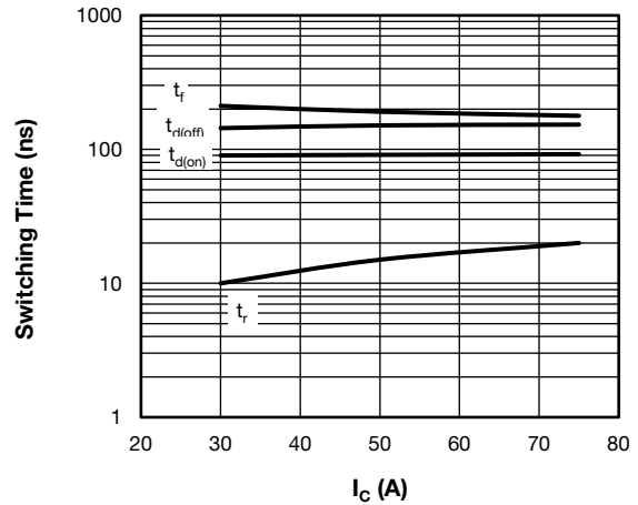
Fig. 8 - Typical Trench IGBT Switching Time vs. I_C (with Antiparallel Diode) T_J = 125^\circ\text{C} , V_{CC} = 600\text{ V} , R_g = 4.7\ \Omega , V_{GE} = +15\text{V}/-15\text{V} , L = 500\ \mu\text{H}
