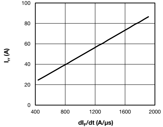
Fig. 14 - Typical Diode I_{rr} vs. dl_F/dt V_{CC} = 400 \text{ V} ; V_{GE} = 15 \text{ V} ; I_{CE} = 5.0 \text{ A} ; T_J = 150 \text{ °C}
