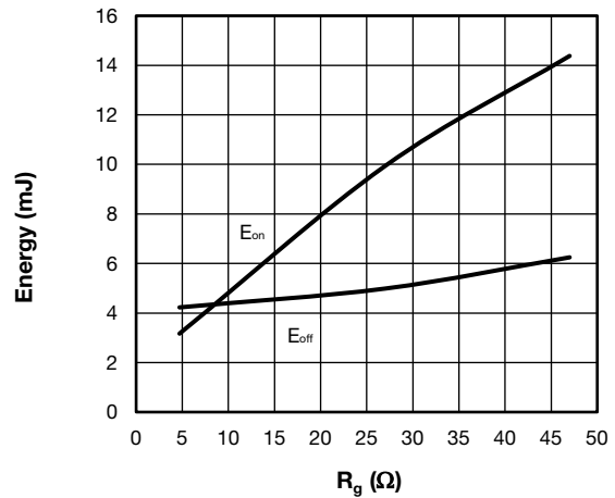
Fig. 9 - Typical Trench IGBT Energy Loss vs. R_g (with Antiparallel Diode) T_J = 125^\circ\text{C} , V_{CC} = 600\text{ V} , I_C = 75\text{ A} , V_{GE} = +15\text{V}/-15\text{V} , L = 500\ \mu\text{H}
