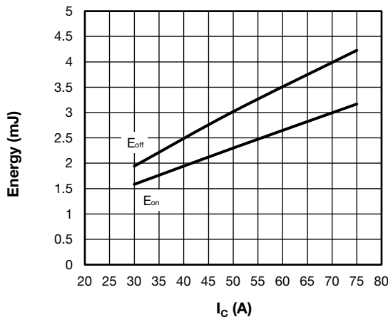
Fig. 7 - Typical Trench IGBT Energy Loss vs. I_C (with Antiparallel Diode) T_J = 125^\circ\text{C} , V_{CC} = 600\text{ V} , R_g = 4.7\ \Omega , V_{GE} = +15\text{V}/-15\text{V} , L = 500\ \mu\text{H}
